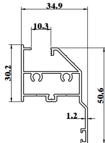
CW646G WEIGHT : 0.568 KG/M AP : 250.83mm
