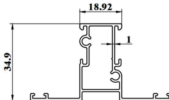
CW6424C WEIGHT : 0.525 KG/M AP : 257.85mm
