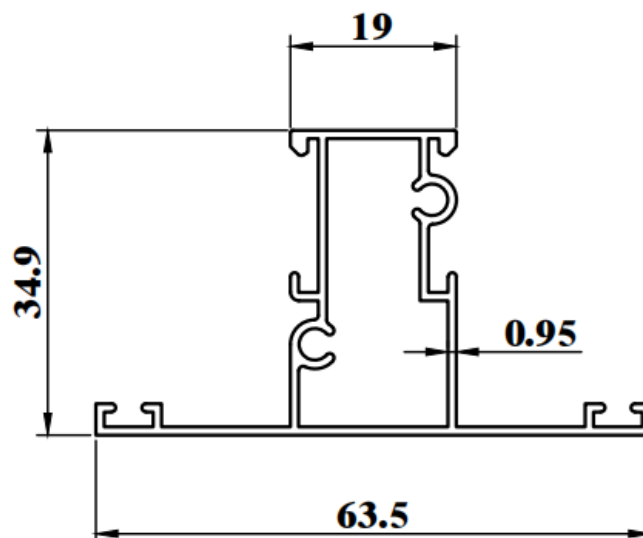
CW762B WEIGHT : 0.507 KG/M AP : 261.55mm
